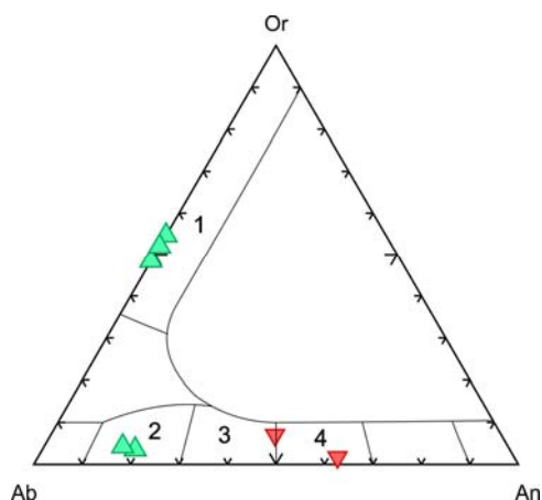
Fig. 12.: Feldspar compositions of NUH-V1 basalt flake (red triangle) and NUH-H1 phonolite flake (green triangle): 1: sanidine, 2: oligoclase, 3: andesine, 4: labradorite.
